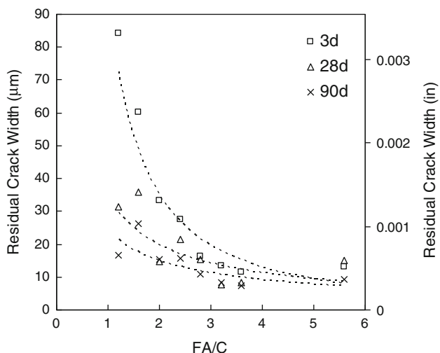
Fig. 11 Residual crack width of HFA ECC as a function of fly ash content at different ages
